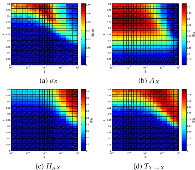
Figure 1: Measures of dynamics versus r and \gamma for K = 4 (color online). Ordered dynamics occur for low r and \gamma (bottom left), and chaotic dynamics for high r and \gamma (top right); the critical regime at the maxima in (a) separates these.
